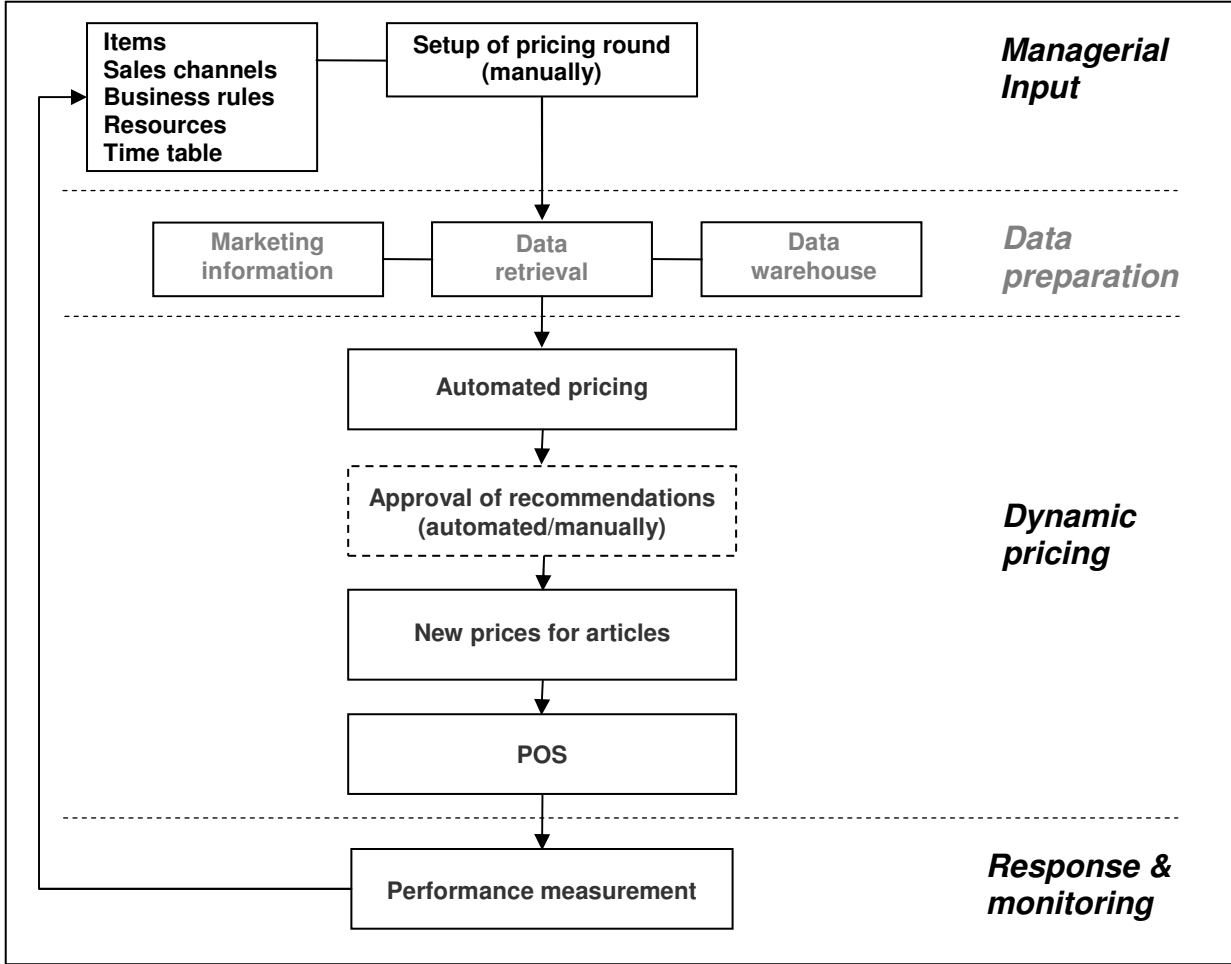
Figure 3: Pricing process
